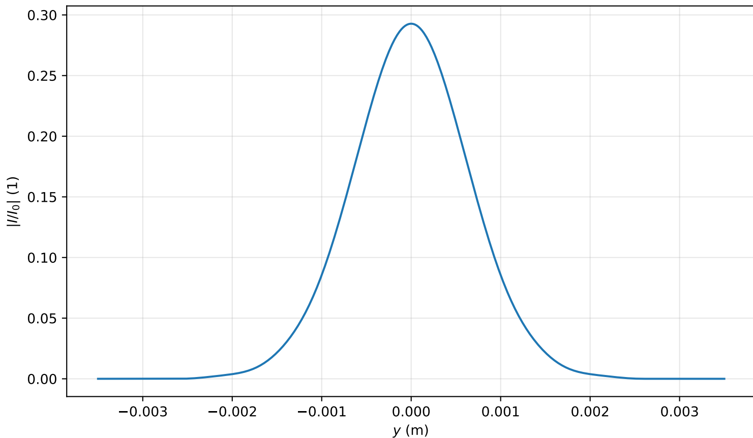
Intensity profile I(x=0, y, z=3.901)/I_0 , P_{in}=0.3P_{cr} , artificial time
